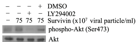
Figure 2. Survivin induced Akt phosphorylation via PI3K. L929 cells were pretreated with/without 50 \mu M LY294002 for 2 hours prior to infection with/without 75 \times 10^7 viral particle/ml retrovirus of Survivin for 48 hours as indicated in the panel. Cells were lysed and immunoblotted using anti-Akt or anti-phospho-Akt (Ser473) antibody. DMSO was used as negative control. Detailed procedures are described in "Materials and Methods". Each panel shows the typical result of 3 independent results.
